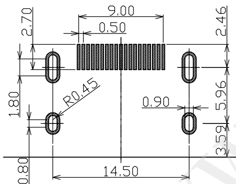
PCB LAYOUT(TOP VIEW T1.6)
